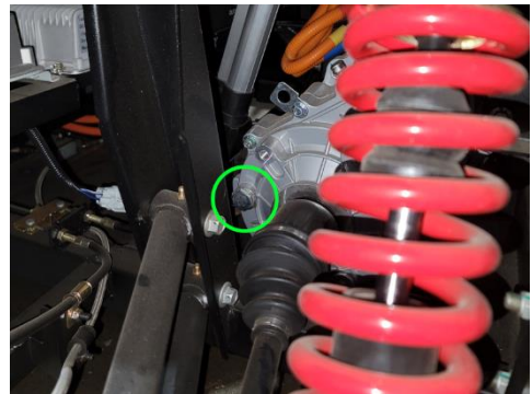
Rear gearbox oil fill plug location (Shown from rear driver side wheel well)
